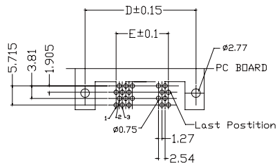
Recommended PCB Layout 26,50P (PCB TOLERANCE±0.05)
