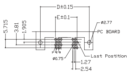
Recommended PCB Layout 68P (PCB TOLERANCE±0.05)
